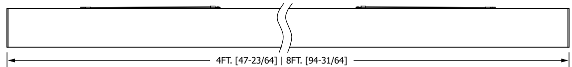
SIDE VIEW
